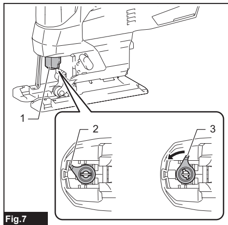
Fig. 7 ▶ 1. Jig saw blade holder 2. Blade clamp lever (released position) 3. Blade clamp lever (fixed position)
